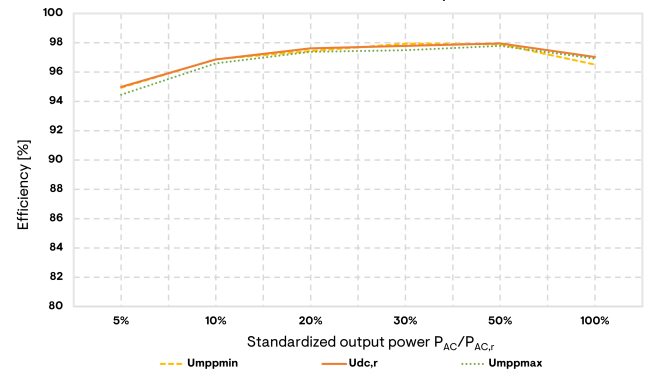
IQ9N Microinverter efficiency curve
